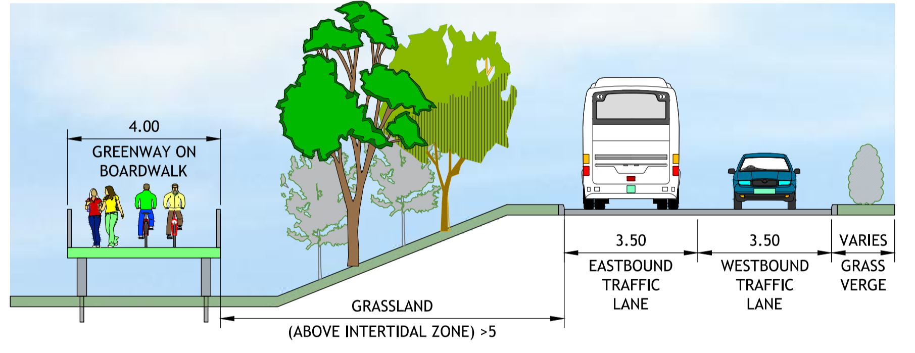
TYPICAL CROSS SECTION TYPE D-3 (CH 3096-3680)
