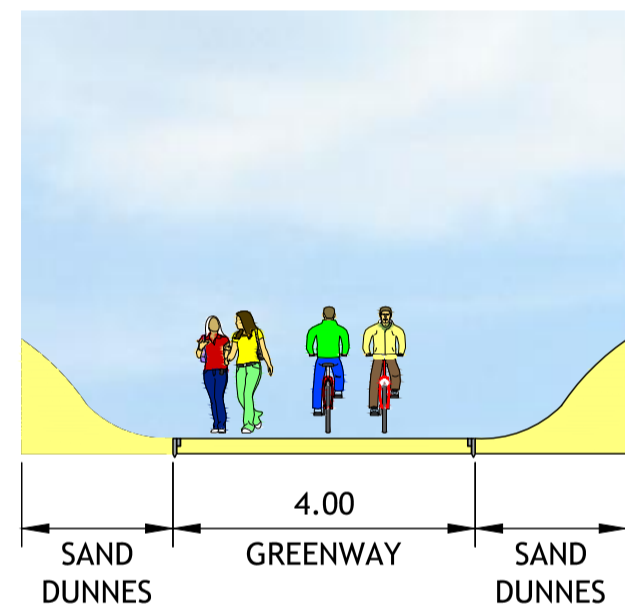
TYPICAL CROSS SECTION TYPE C (CH 5890-6445)
