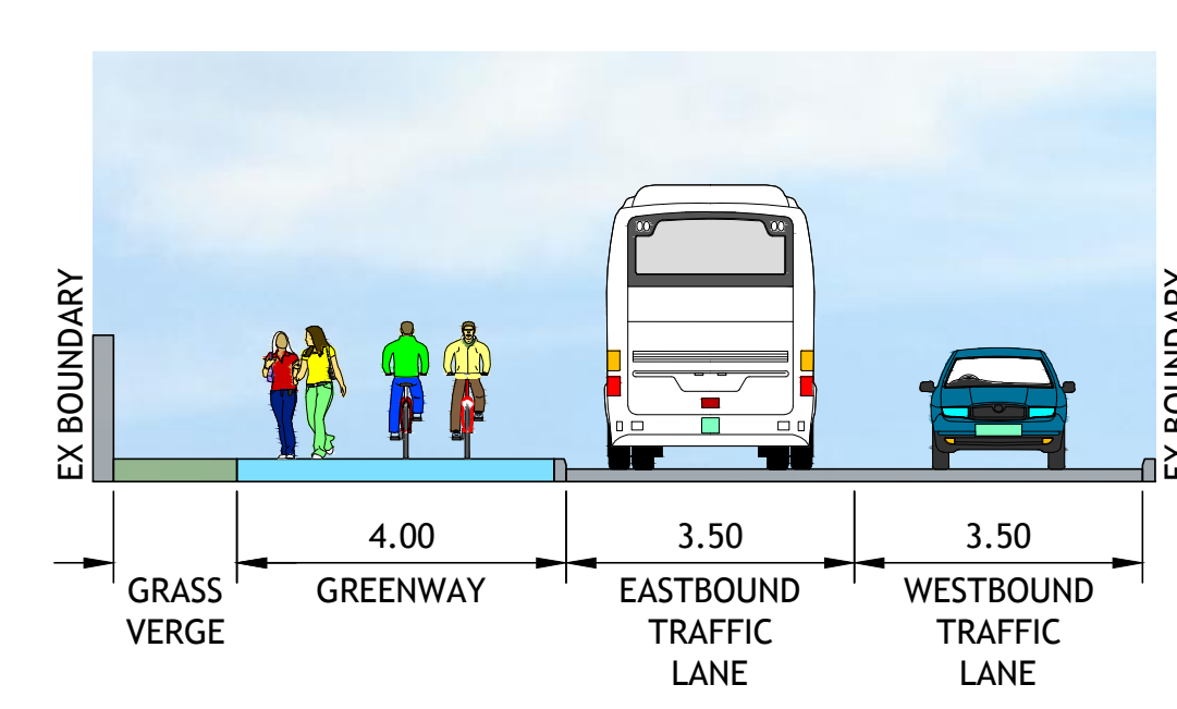
TYPICAL CROSS SECTION TYPE A-1 (CH 600 TO CH 740)
