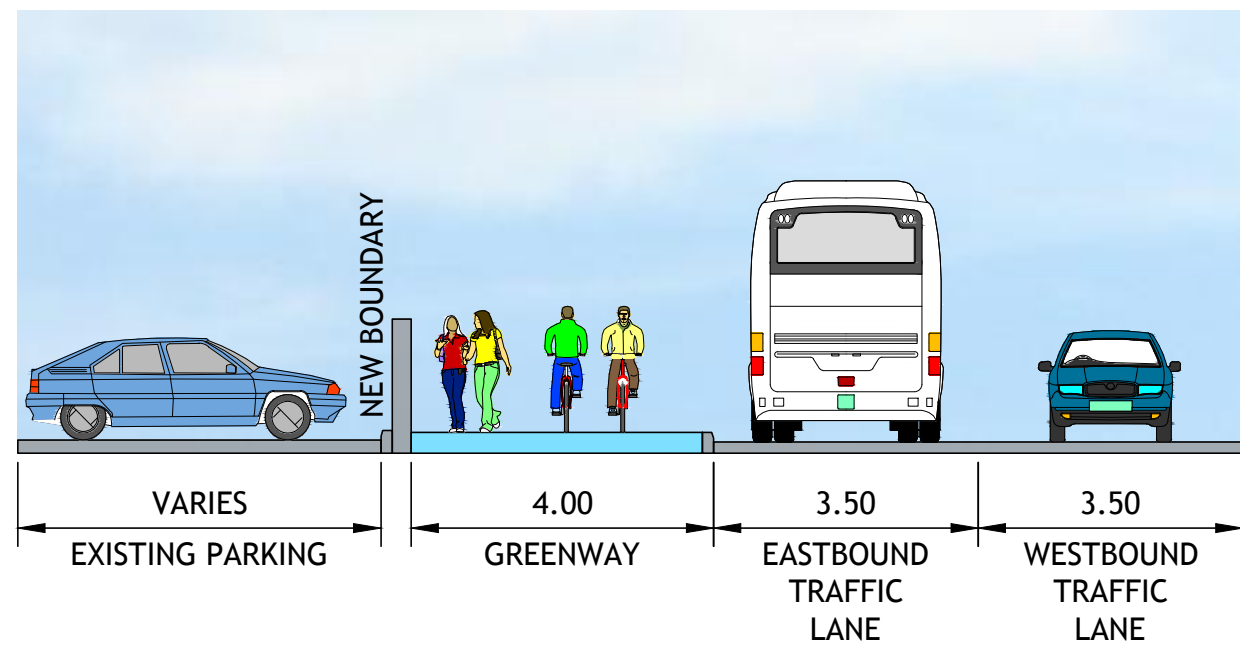
TYPICAL CROSS SECTION TYPE A-1 (CH 740 TO CH 800)
