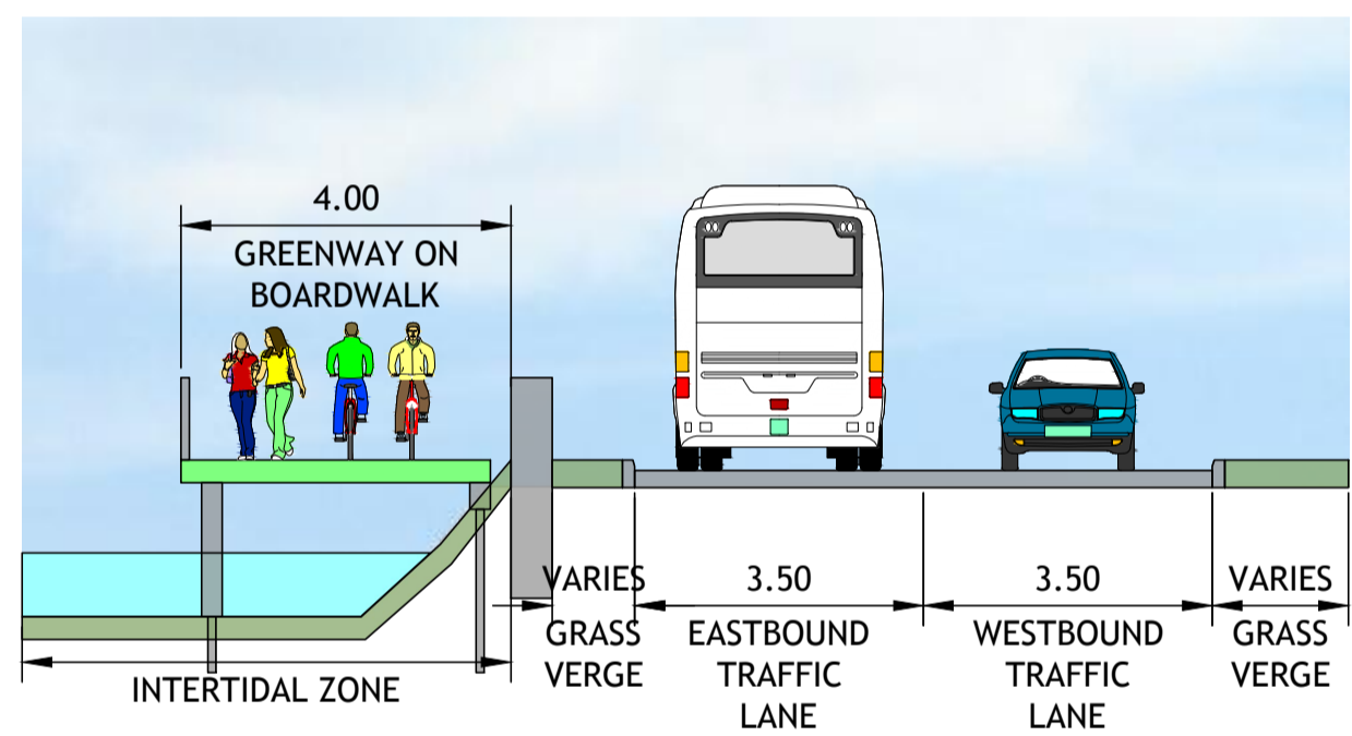
TYPICAL CROSS SECTION TYPE C-2 (CH 2000-2100)
