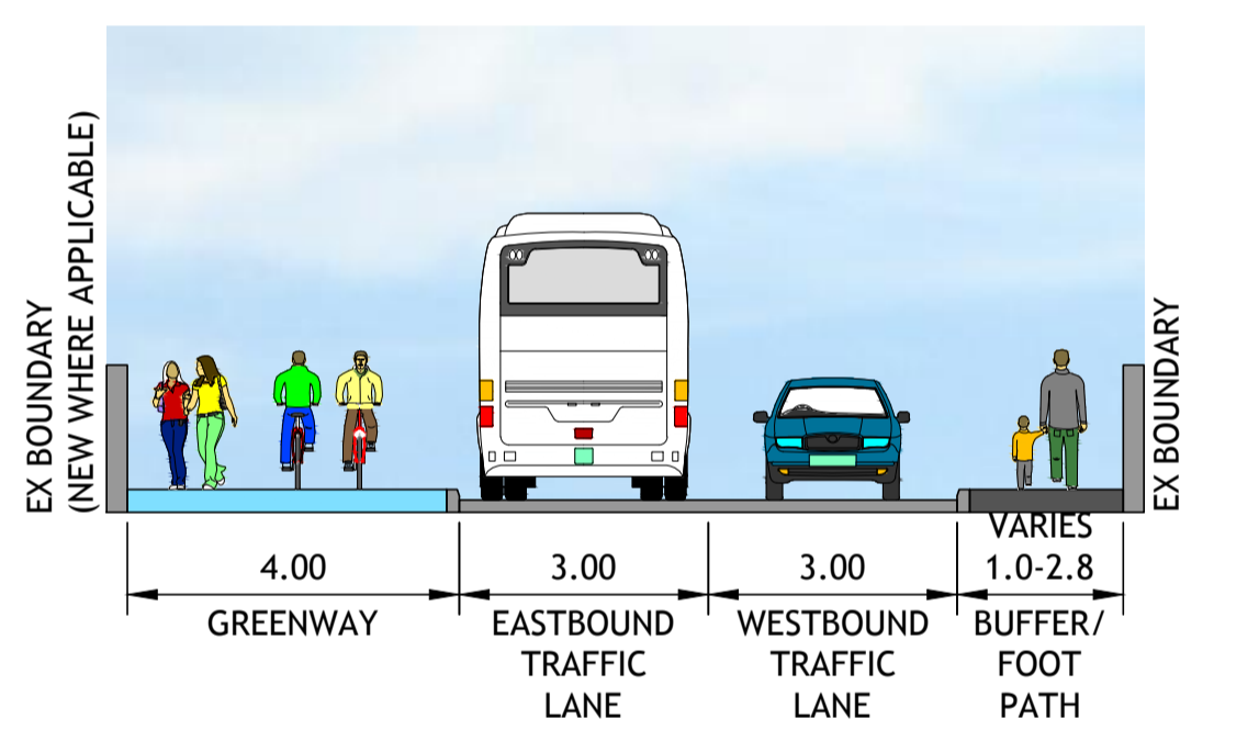
TYPICAL CROSS SECTION TYPE A-3 (CH 5130-CH 5220)
