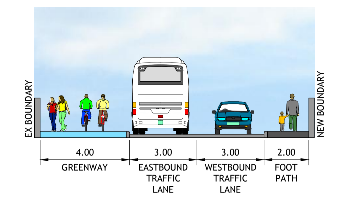
TYPICAL CROSS SECTION TYPE A-4 (CH 5220-CH 5250)
