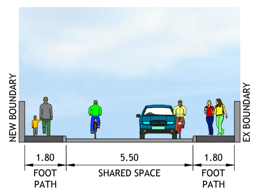
TYPICAL CROSS SECTION SHARED STREET (CH 5730)
