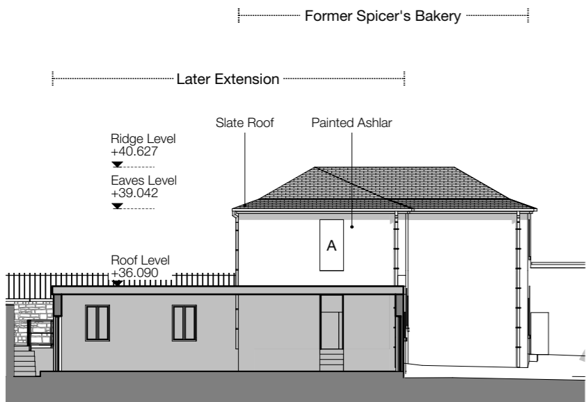
Existing Rear Elevation 1:200
