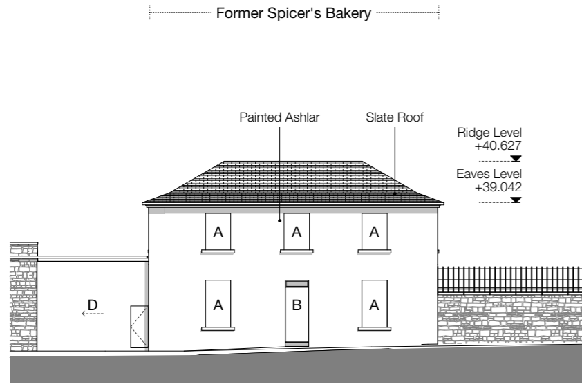
Existing Front Elevation 1:200
