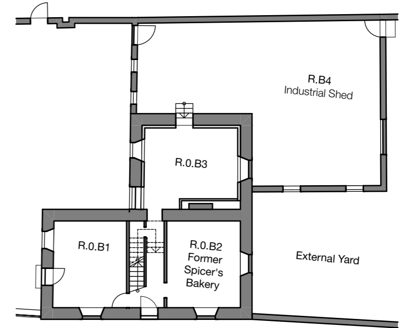
Existing Ground Floor Plan 1:200
