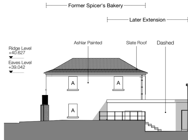
Existing East Elevation 1:200
