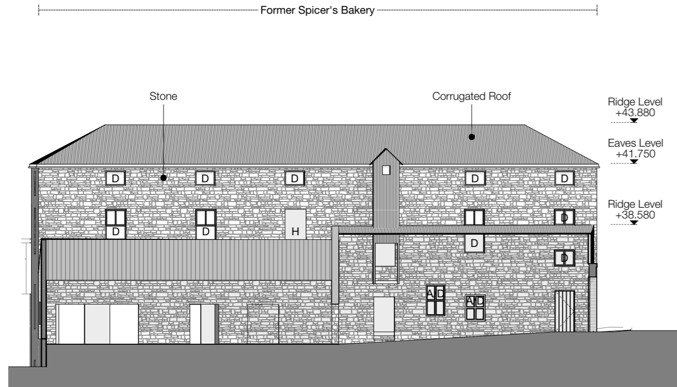
Existing Spicer's Mill West Elevation 1:200
