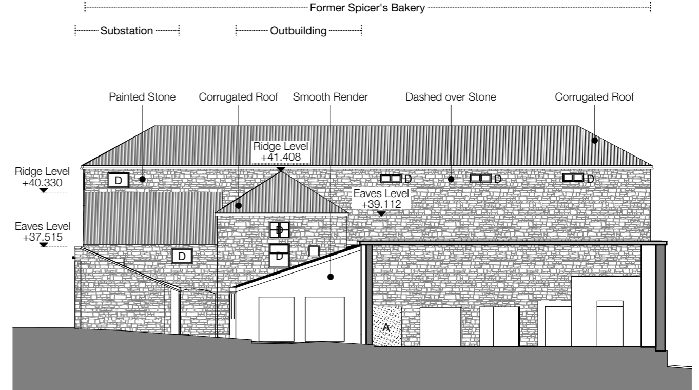
Existing Spicer's Mill East Elevation 1:200
