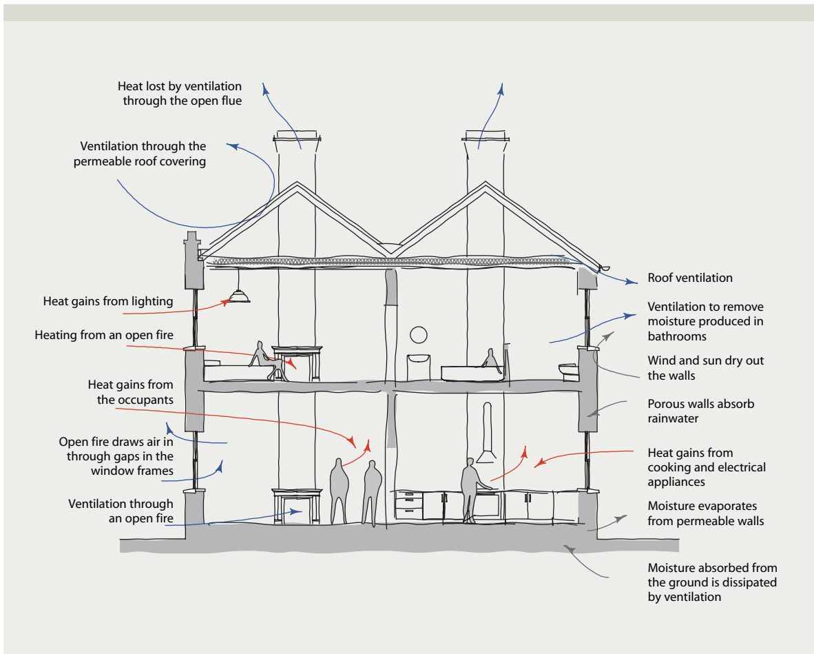
A comparison of the ventilation and heating requirements for a traditional building (above) and a modern building (below)
