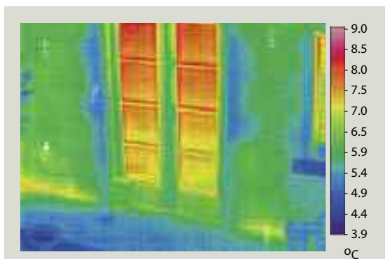
A thermographic image of a double-glazed door at semi-basement level in a nineteenth-century terraced house; note how the yellow patches at the base of the wall, which are damper, indicate that these areas are emitting heat at a higher rate than the rest of the wall
